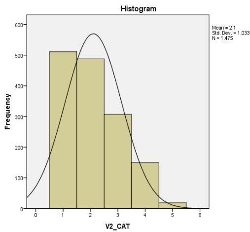
Figure 108: Low-fare airline
