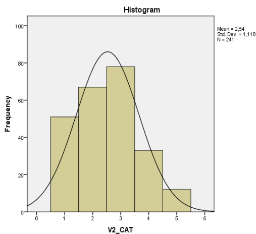
Figure 112: Cargo airline
