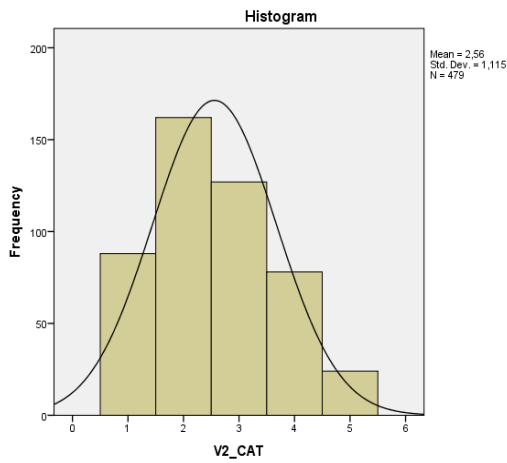
Figure 110: Regional airline
