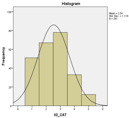
Figure 111: Charter Airline
