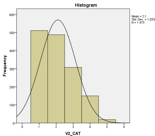
Figure 137 Low-fare airline
