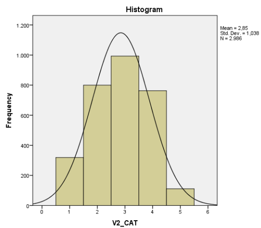
Figure 109: Network airline
