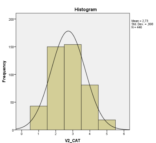
Figure 113: Business aviation
